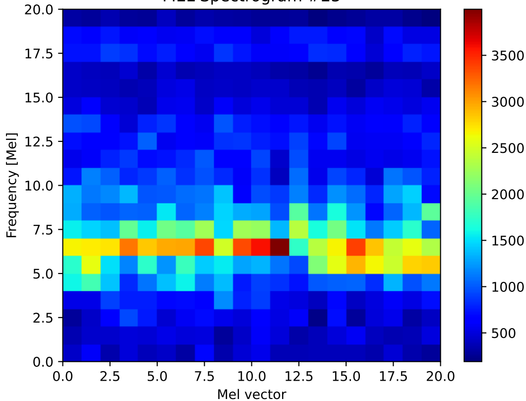
MEL Spectrogram #23
